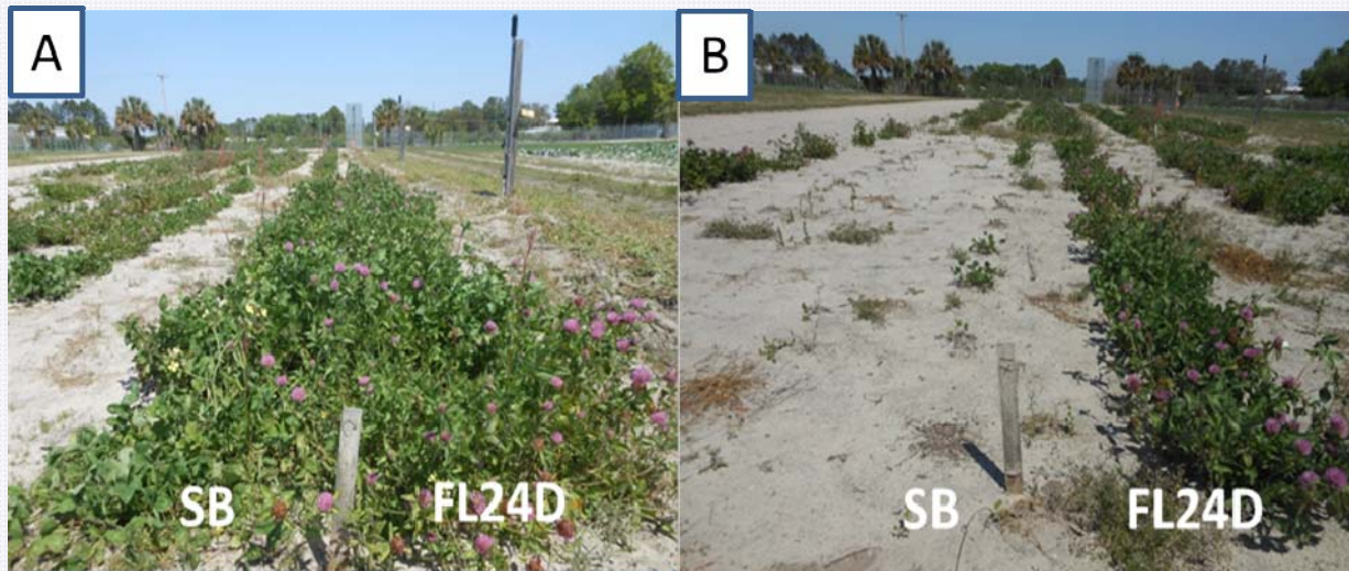
Figure 1. Response of 'FL24D' and Southern Belle (SB) to 2,4-D. A) Control Treatment (No spraying); B) Spraying with recommended rate of 2,4-D ( x=1.06 \text{ kg ha}^{-1} ). Herbicide applied on Jan. 16, 2013 and photo taken on March 28, 2013.
